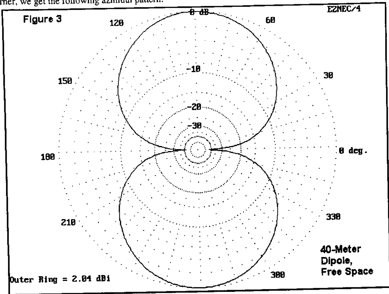
Fig. 3. Free space azimuth pattern of a dipole.
