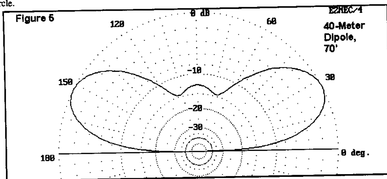
Fig.5. Elevation pattern of a 40-meter dipole at 70' height along the azimuth of maximum radiation.
